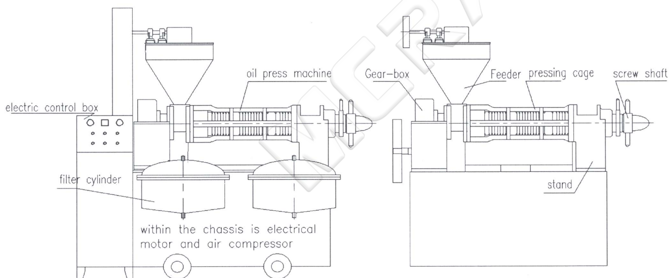
Structure diagram of oil press machine
